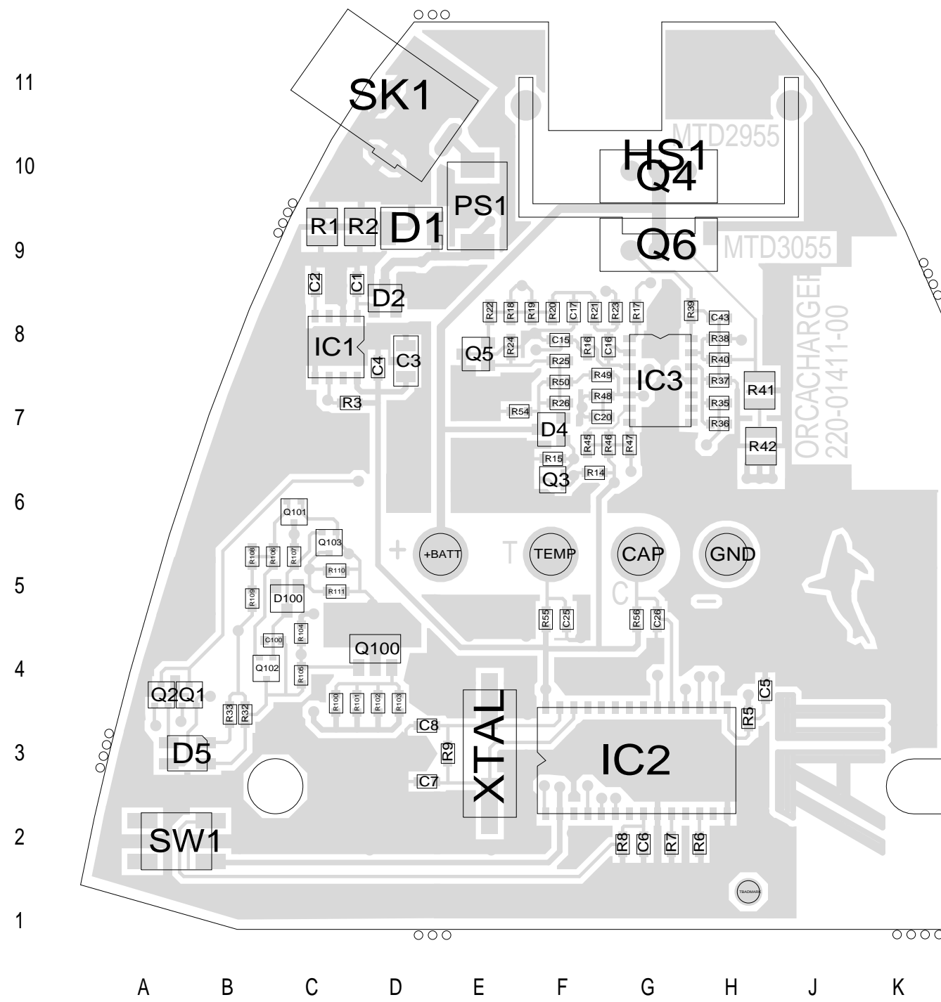
220-01411-00 TOP COPPER
